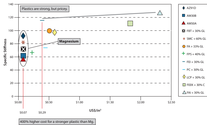
Figure 5 – Specific Strength & Price of Materials.
